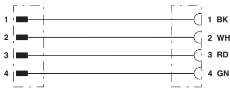
Contact assignment of 7/8" plugs/sockets
