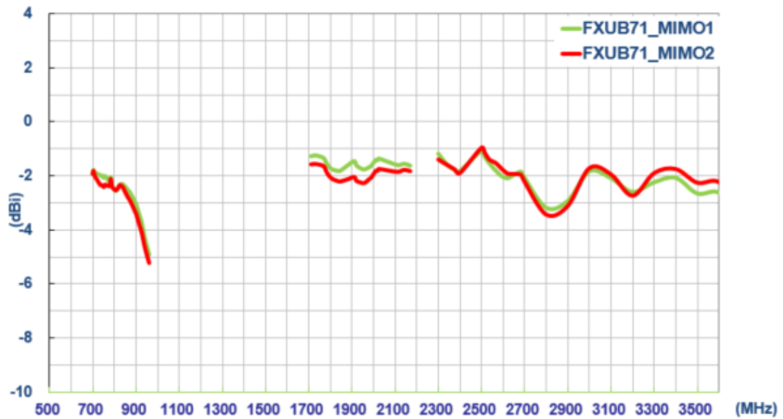
Figure5. Average gain with 150 mm cable length and on the 2mm ABS of FXUB71
